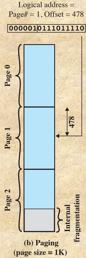
Figure 7.11 Logical Addresses
