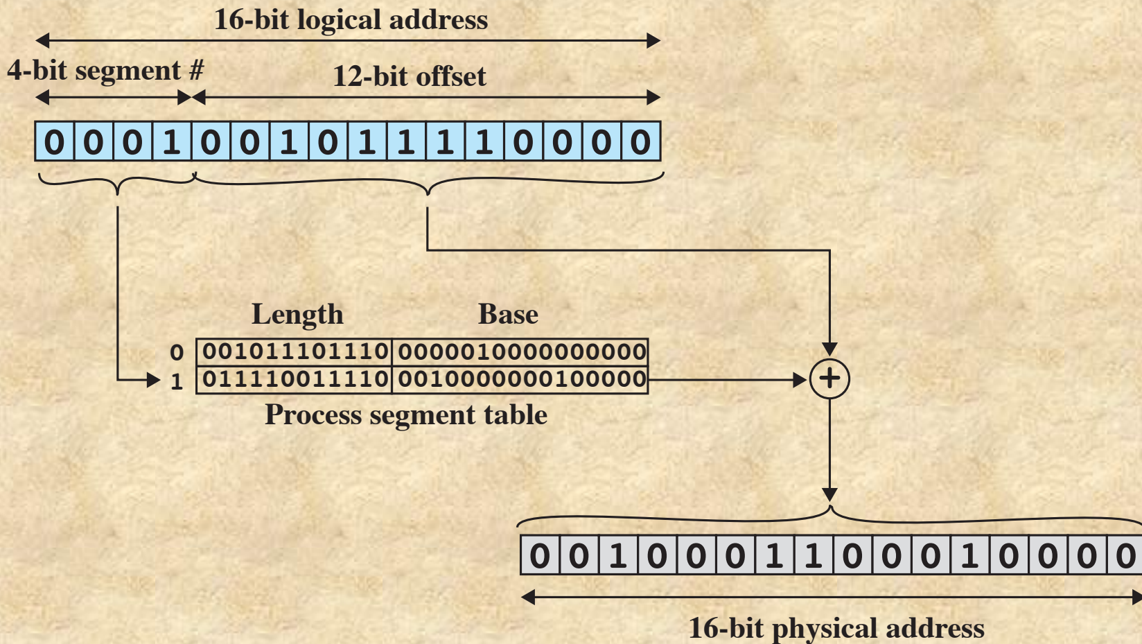
(b) Segmentation
