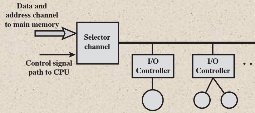
(a) Selector
