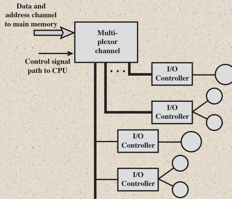
(b) Multiplexor
