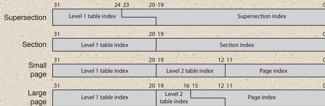
(c) Virtual memory address formats
