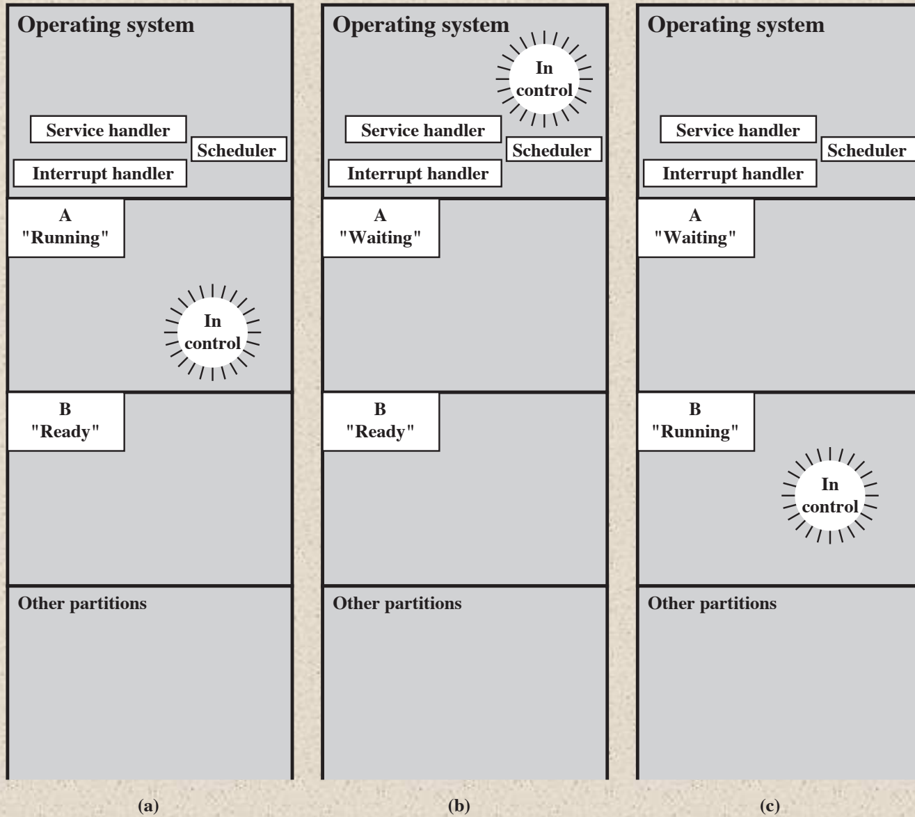
Figure 8.9 Scheduling Example
