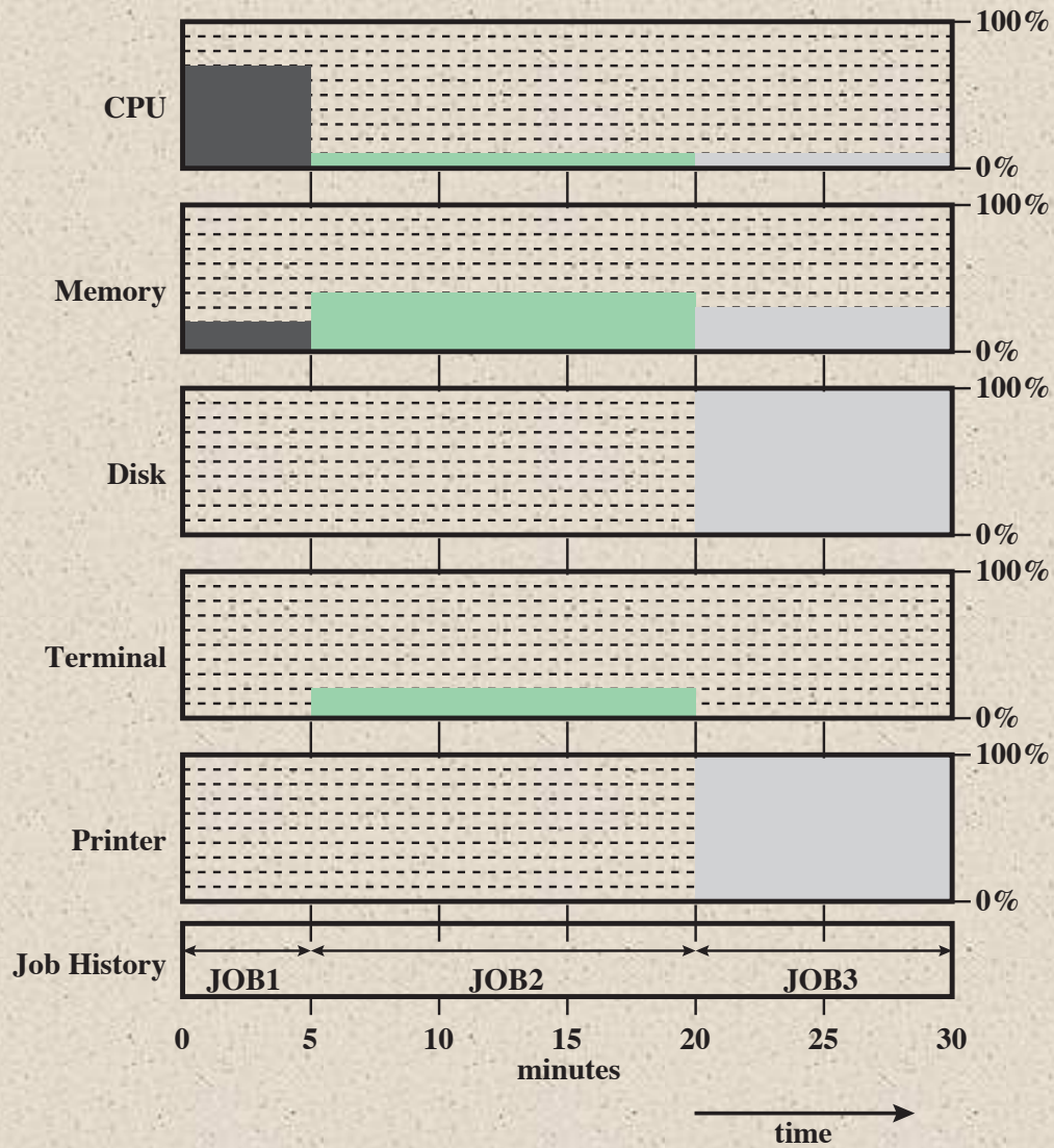
(a) Uniprogramming
