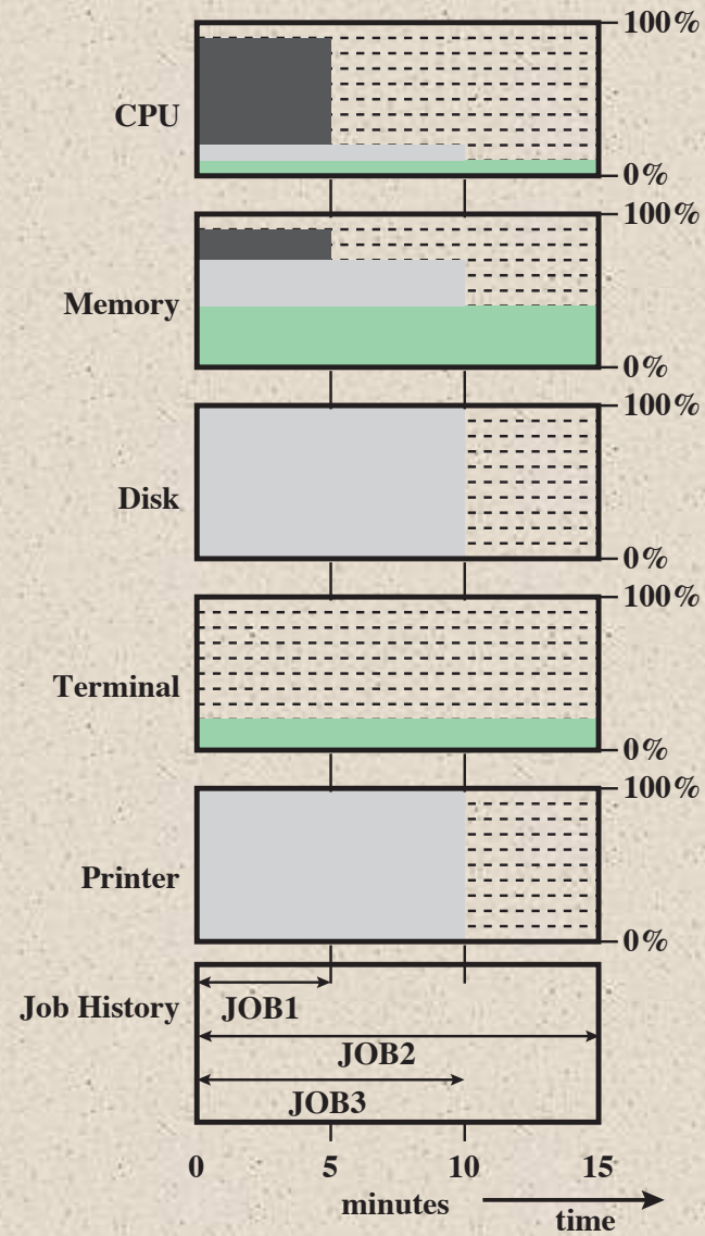
(b) Multiprogramming
